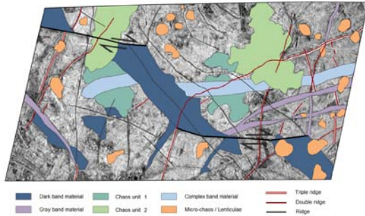
Figure 1: Geological map of Europa with the different chaos units (green toned) and their relations with other geologic units. The section corresponds to the mosaic of images E14ESWEDGES01 (14th Galileo orbit).
