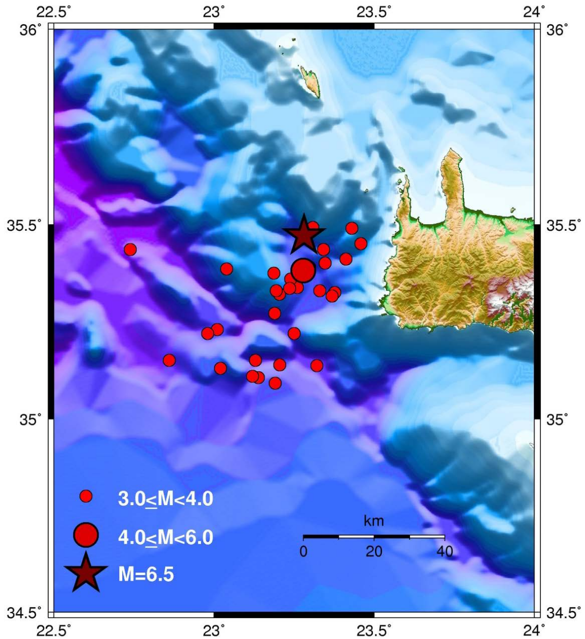
Figure 3. Geographical distribution of the aftershocks (which were recorded up to the end of November 2013, red circles) of the October 12, 2013, M=6.5 mainshock (denoted by a star) which occurred in the SW part of the Hellenic arc, ~20km off the west coast of Crete
