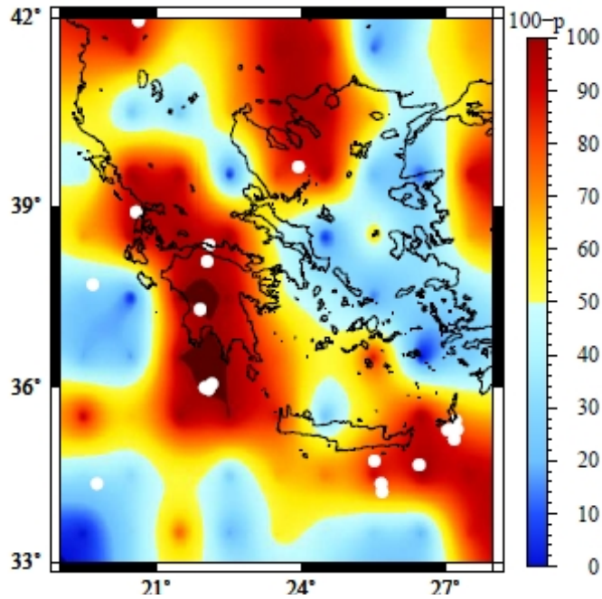
Figure 10. Compliance parameter p of the Lunar Monthly Synodic tidal period for the year 2000. White marks indicate Earthquake epicenters: circles 4.5 < M < 5.5 , stars M \geq 5.5
