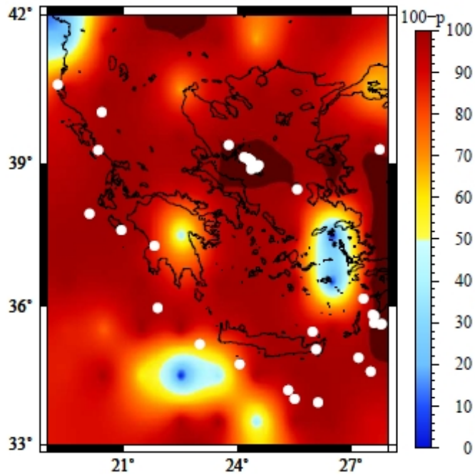
Figure 11. Compliance parameter p of the Lunar Monthly Synodic tidal period for the year 2001. White marks indicate Earthquake epicenters: circles 4.5 < M < 5.5 , stars M \geq 5.5
