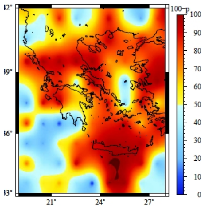
Figure 6. Compliance parameter of the Lunisolar diurnal K1 tidal period for the time period January,2005- December, 2015.
