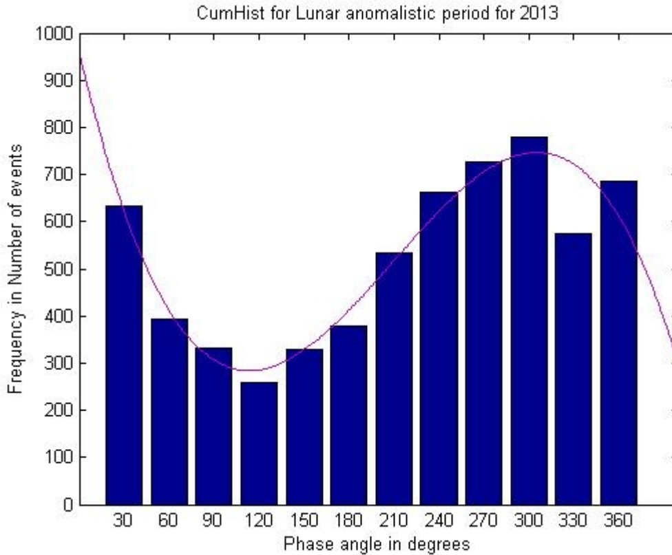
Figure 1. Cumulation Histogram for the Anomalistic Monthly period for 2013
