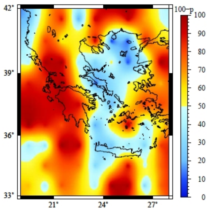
Figure 7. Compliance parameter of the Lunisolar diurnal O1 tidal period for the time period January, 2005- December, 2015.
