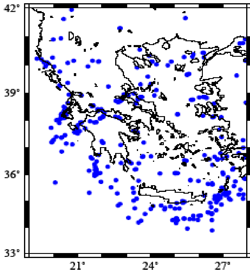
Figure 3. Earthquake with M > 4.5 occurred in the area of Greece between January 2005 and December 2015
