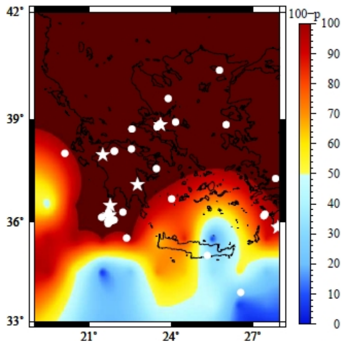
Figure 18 Compliance parameter p of the Lunar Monthly Synodic tidal period for the year 2008. White marks indicate Earthquake epicenters: circles 4.5 < M < 5.5 , stars M \geq 5.5
