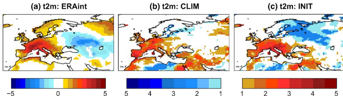
a Observed anomalies of t2m for 2003 JJA (K). Dots indicate where the anomaly is in the upper quintile (estimated over 1981–2010). b t2m odds ratio for seasonal forecasts initialised on May-01 with climatological soil moisture conditions (CLIM). c Same as b , but for forecasts initialized with observed soil moisture anomalies.
