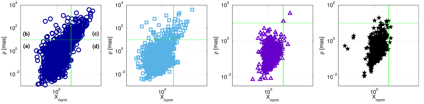
Fig. 3. Angular separation \rho against the normalized separation X_{\text{norm}} for (from left to right) VIE (dark blue), GFZ (light blue), K band (purple), and XK\alpha (black) with respect to GSF. The vertical line is located at X_{\text{norm}} = 4.1 , the horizontal at \rho = 10 mas.
