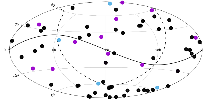
Fig. 1. Sources unique to one catalog. Light blue: GFZ, purple: K band, and black: XK\alpha .
