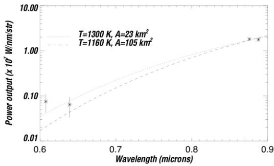
Figure 1: Brightness of Tvashtar as a function of effective wavelength as measured from LORRI and MVIC observations. Two blackbody curves are also shown.
