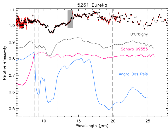
Figure 2. Spitzer IRS Spectrum of 5261 Eureka and RELAB spectra of angrites [3]. The olivine-rich meteorites (Fig. 1) provide a better spectral match to the reststrahlen features in the IRS data than do these basaltic meteorites.
