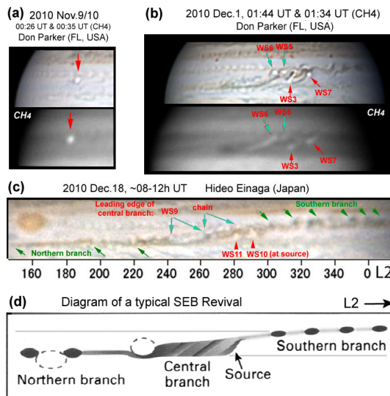
Fig.1. Appearance of the SEB Revival. South is up. (a) Nov.9/10: The initial bright plume, 12 hrs after its first appearance: Visible and methane band ( 0.89 \mu\text{m} ) images. (b) Dec.1: Two subsequent bright plumes which arose at the source (red arrows) and two which arose in the leading edge (cyan arrows). All are methane-bright. (c) Dec.18 (cylindrical projection): Structure of the expanding Revival. (d) Diagram of a typical SEB Revival [ref.1].
