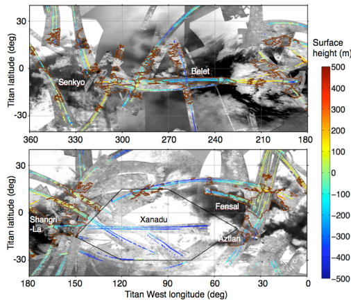
Figure 2: Global view of Titan's SAR-derived surface heights overlaid on SAR imagery and ISS base map. Dune regions are outlined in brown.
