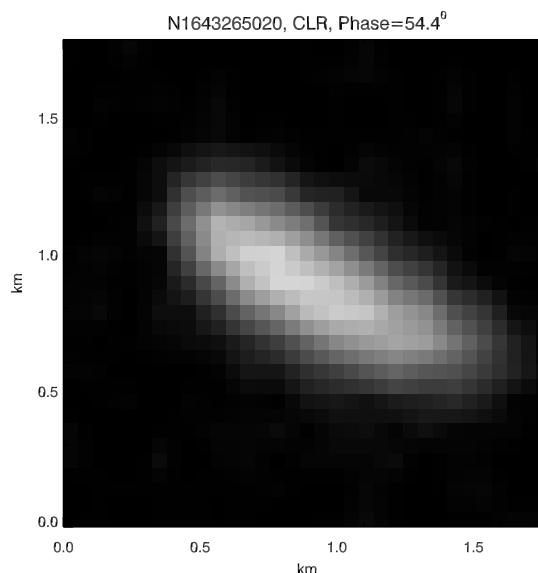
Figure 1: Image of Aegaeon obtained during the close encounter on January 27, 2011. The raw imaging data have been re-sampled by a factor of two in this image for the sake of clarity. The elongated shape of the moon is clearly evident.
