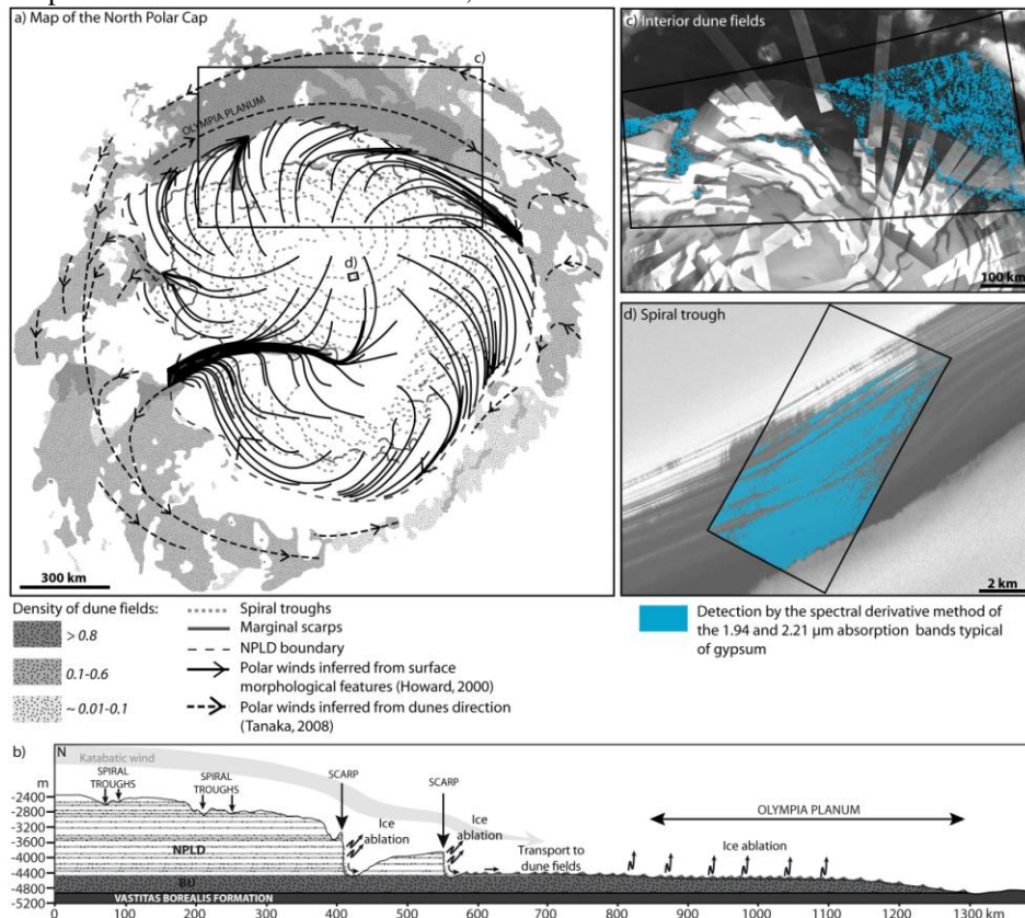
Figure 1: a) Map of the north polar dune fields, spiral troughs and marginal scarps with superimposition of the polar winds. b) Interpretative scenario for the formation of superficial gypsum bearing sediment in the North Polar Cap. c) and d) Distribution of gypsum respectively on the interior and circumpolar dune fields, and on dust veneer.
