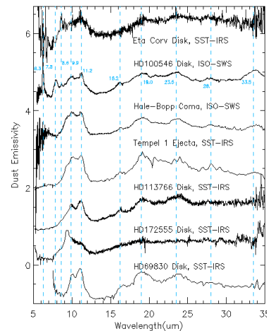
Figure 2 – Comparison of the mid-IR spectra of \eta Corvi with the spectra of dust from: a young, organic rich Herbig A0 star building a giant planet (HD100546) [5]; two comets (Hale-Bopp and Tempel 1) [5]; a young F5 star building a terrestrial planet (HD113766) [6]; the silica-rich debris created by a hypervelocity impact in the HD172555 system [7]; and a mature main sequence star with a dense zodiacal cloud (HD69830) [8]. The similarity between the \eta Corvi and HD100546 spectra is readily apparent.
