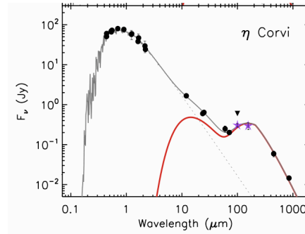
Figure 3. SED for \eta Corvi showing the 0.4 – 2.2 \mu m BVR/2MASS system photometry dominated by stellar photospheric emission, the stellar/circumstellar dust MIR flux measurements of IRAS and Spitzer, & the cold FIR excess measured by Herschel and JCMT/SCUBA [2]. Solid grey line: combined fit to the \eta Corvi SED using a 2-blackbody model (red) with warm (350K) & cold (35K) dust reservoirs + emission from a Kurucz F2V photosphere (dashed line).
