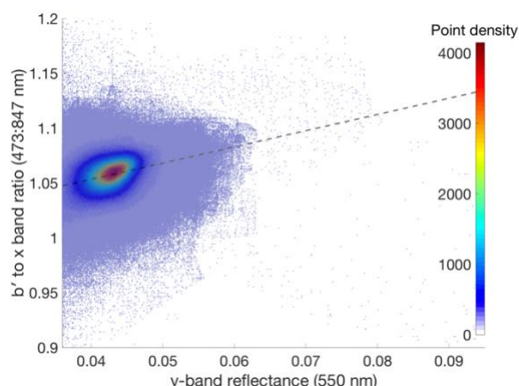
Figure 1. The b'/x band ratio (473:847 nm) versus normal reflectance at 550 nm across Bennu. In general, higher-albedo areas correlate with bluer materials, as indicated by the best-fit dashed line, but other populations of material are also evident.
