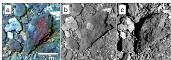
Figure 2. [a] Color and albedo variation across a single boulder ( -5^\circ , 250^\circ ). MapCam x/b' and b'/v band ratio images acquired at 7^\circ phase angle (25 cm/pix). Here, negative-sloped areas appear blue and positive-sloped areas appear red. [b] A higher-resolution PolyCam image of this boulder acquired at a similar phase angle as panel a (7 cm/pix). [c] The same boulder acquired by PolyCam at a 40^\circ phase angle at the opposite side of the subsolar point (5.5 cm/pix). Differences in texture and relief on the bright area of this boulder are more visible at these illumination conditions.
