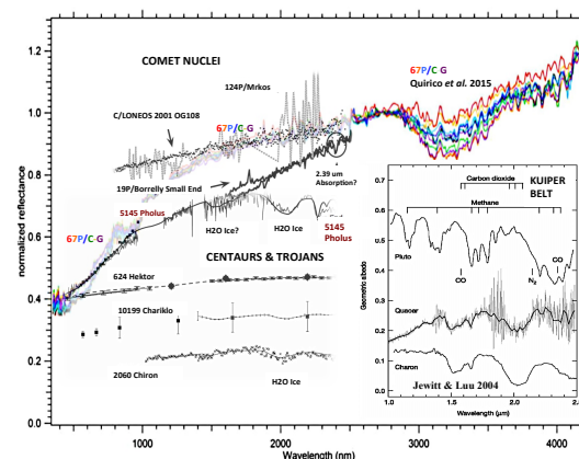
Figure 1: Compendium of NIR reflectance spectra for Solar System comets, Centaurs, and Trojan small bodies, as published in [4]. Centaur Pholus, which is relatively good match for MU69 spectrally, is commonly known as the 'reddest object in the solar system', but in reality is only very red from 0.4 - 1.5 \mu m. Longwards of 1.5 \mu m H 2 O ice absorption on its surface takes over and the reflectance becomes flat to slightly blue with increasing wavelength. ( Inset ) Typical KBO NIR reflectance spectra, dominated by hypervolatile surface ice absorptions, are grey to slightly blue in the NIR.
