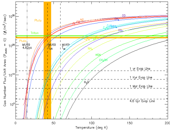
Figure 2 – Production rate of gas molecules, Q_{\text{gas}} , for a pure ice species vs ambient temperature, after [3]. The curves are controlled by the Vapor Pressure vs Temperature behavior for an ice. The dashed horizontal lines show the maximal Q_{\text{gas}} for which any appreciable solid ice will remain in a zero Pa environment. Above these lines, Q_{\text{gas}} * \Delta(\text{Time}) > the molar surface density of an ice, \sim 10^{19}/\text{m}^2 . The MU69 flyby showed no evidence for pure hypervolatile ices in abundance today on the surface of MU69, consistent with the very short predicted residence times for pure hypervolatile ices (red curves) at current KB temperatures. By contrast, at the \sim 10 uBar surface of Pluto, the recondensation rate for hypervolatile ice (yellow horizontal line) can match its sublimation rate, and solid ice can coexist with atmospheric gas.
