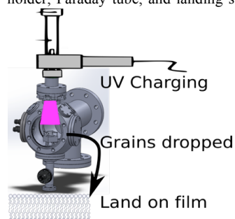
Figure 2: Computer generated drawing of the charging chamber and conceptual design of the experiment. Grains are charged during exposure to UV light or electrons from a filament source and then transported and dropped onto the organic films where the effects are measured.
