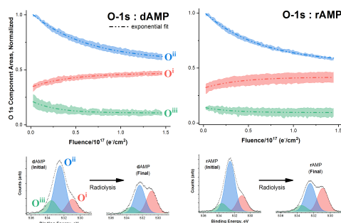
Figure 1 XPS study of LEE damage of rAMP and dAMP nucleotides. The decrease in the O^{ii} peak signifies breaking of the sugar subunit, while growth in O^i implies formation of phosphate oxygen.
