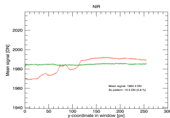
Figure 2: Example of stray light pattern removal for NIR filter. The red curve is the averaged y-profile (over all columns and framelets) before correction. The green curve is the result of the subtraction of the fixed stray light pattern with adjusted intensity. The maximum amount of stray light removed here is 0.8% of the measured signal.
