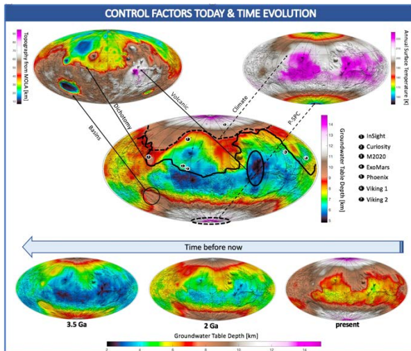
Figure 1: The upper image shows for one selected standard run the depth of the theoretical cryosphere/liquid water table interface (DH 2 O), below which pure groundwater could exist today. This depth depends on surface temperature and on local heat flux. The lower image shows how the cryosphere/liquid water table interface changed through time assuming no changes in crustal thicknesses, crustal properties, or climate.
