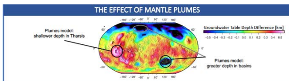
Figure 1: Map of the differences between a 3D spherical full mantle convection model with and without plumes.
