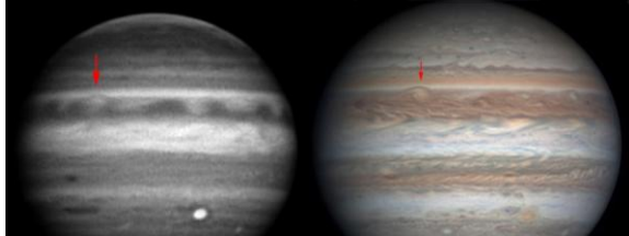
Figure 2. Image at 889 nm showing the high-amplitude methane-dark waves on the NEB, with a visible image (2017 June 14, by C. Go). Red arrow: a long-lived AWO.
