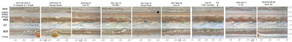
Figure 1. Excerpt from cylindrical maps showing the varying appearance of the NEB from 2016 to 2018. All maps made by M.V. (JUPOS team).
