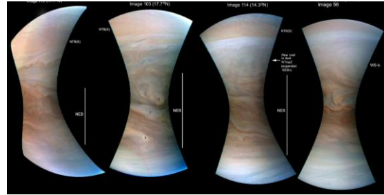
Figure 3. JunoCam images centred on the NEB from PJ3 to PJ6. The images were reprojected as if viewed from a point above the spacecraft's track, with north up.
