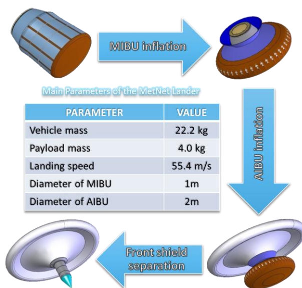
Figure 1: MetNet Precursor Mission main parameters.
