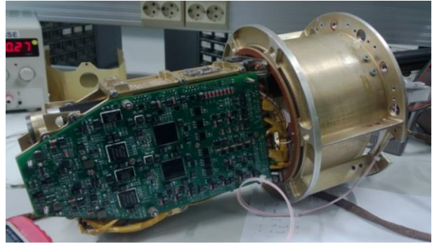
Figure 2: MetNet payload bay electronics in tests.
