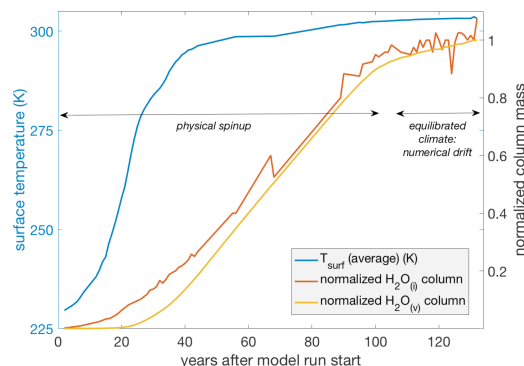
Fig. 1 GCM spin-up for a cold/dry initial condition. The column masses are normalized to values of 120 \text{ pr-}\mu\text{m} for ice and 5 \times 10^4 \text{ pr-}\mu\text{m} for water vapor.
