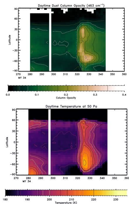
Figure 1: MRO/MCS daytime dust and temperature in the vicinity of the C event. Ls 320 corresponds roughly to 7 Jan 2019 and Ls 340 to 15 Feb.
