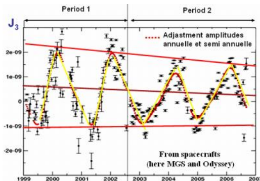
Fig. 3. Expected secular variation of the zonal coefficient J_3 of gravitational field of Mars: \dot{J}_3 \approx -(2 \div 5) \cdot 10^{-11} \text{ 1/yr} (Barkin, 2009).
