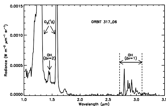
Figure 1: Example of nightside airglow spectrum. The bands between 2.7 and 3.1 \mu\text{m} belong to the \Delta v=1 sequence of the OH Meinel bands, while the \Delta v=2 sequence can be identified from 1.40 to 1.49 \mu\text{m} [1].
