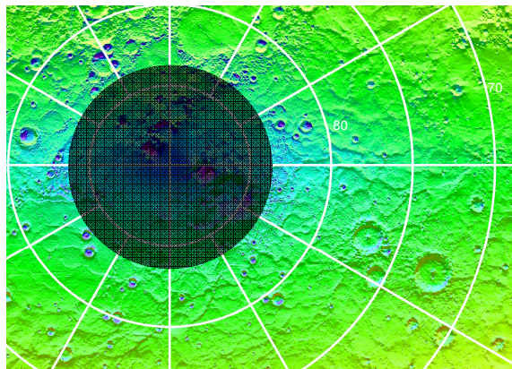
Figure 1. Model-calculated annual average temperatures in the north polar region of Mercury
