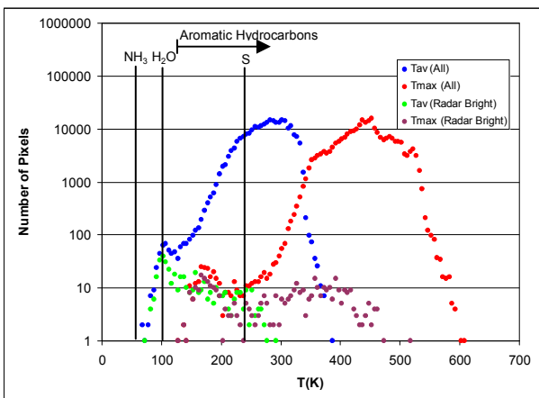
Figure 2. Histograms of annual average and annual maximum surface temperatures for all the areas, and separately for radar-bright areas. The volatility temperatures of ammonia, water ice, sulfur, and aromatic hydrocarbons are also indicated [9,10].
