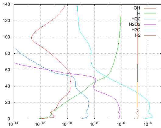
Figure 2: Annual average profiles of \text{HO}_x species volume mixing ratios vs. height in km.
