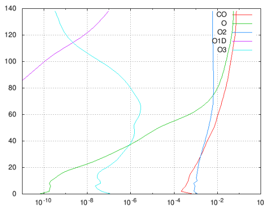
Figure 3: Annual average profiles of \text{O}_x species volume mixing ratios vs height in km.
