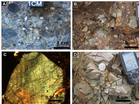
Figure 3. Metamorphism impact figures. A: polymict breccias. B: monomict breccias. C: shocked quartz showing PFs. D: radial fractures.
