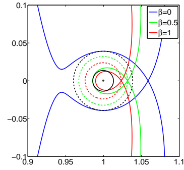
Figure 3: Zero-velocity curves (ZVC) for different values of \beta in the case of HD2094588 b. The dark dotted circle corresponds to the supposed altitude of the exobase, enclosed by the ZVC of the Three-Body problem ( \beta = 0 , blue curves). The green and red curves correspond to ZVC for \beta = 0.5 and \beta = 1 .
