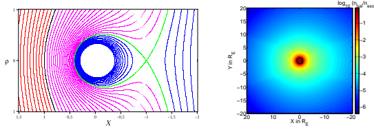
Figure 1: Zero velocity curves (dimension less distance) for our problem and ballistic particles density at Earth for hydrogen and T_{exo} = 800\text{ K}
