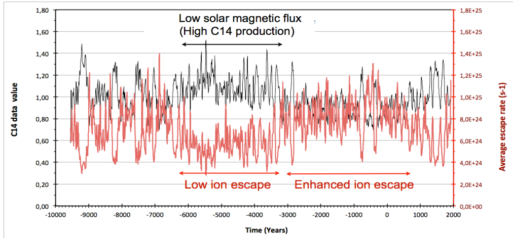
Fig. 2 Long-term (12 000 years) escape rates of the sum of O^+ and O_2^+ from Mars based on C14-data (proxy for the solar magnetic flux).
