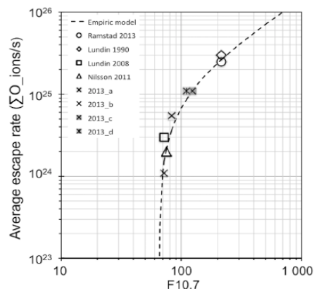
Fig. 1 Regression curve describing the relation between the sum of O + and O 2 + average escape rates versus F10.7.
