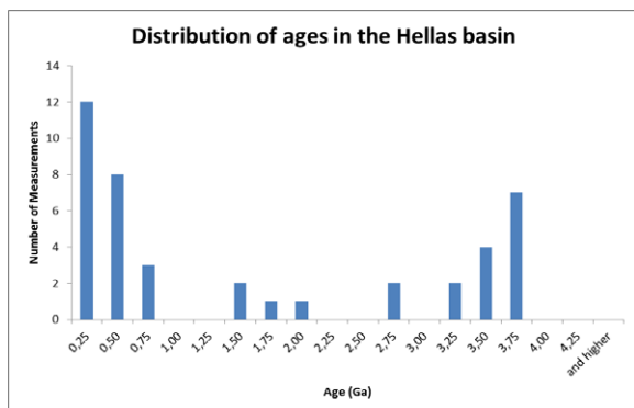
Fig. 3: Age distribution of measured ages in selected counting areas. Ages between 3.2 Ga and 3.75 Ga represent the formation of the basin floor units, younger ages represent the subsequent modification. The abundance of ages between 0.75 Ga and 0.25 Ga indicates a widespread episode of resurfacing of the eastern Hellas ridged plains.
