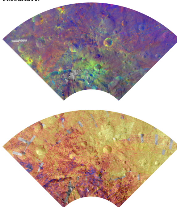
Figure 1: The Sestilia region as seen in: (top) the ratio color composite of the VIR channels at 749/438nm (Red), 749/917nm (Green), and 438/749nm (Blue), and (bottom) the position of the BII pyroxene absorption.
