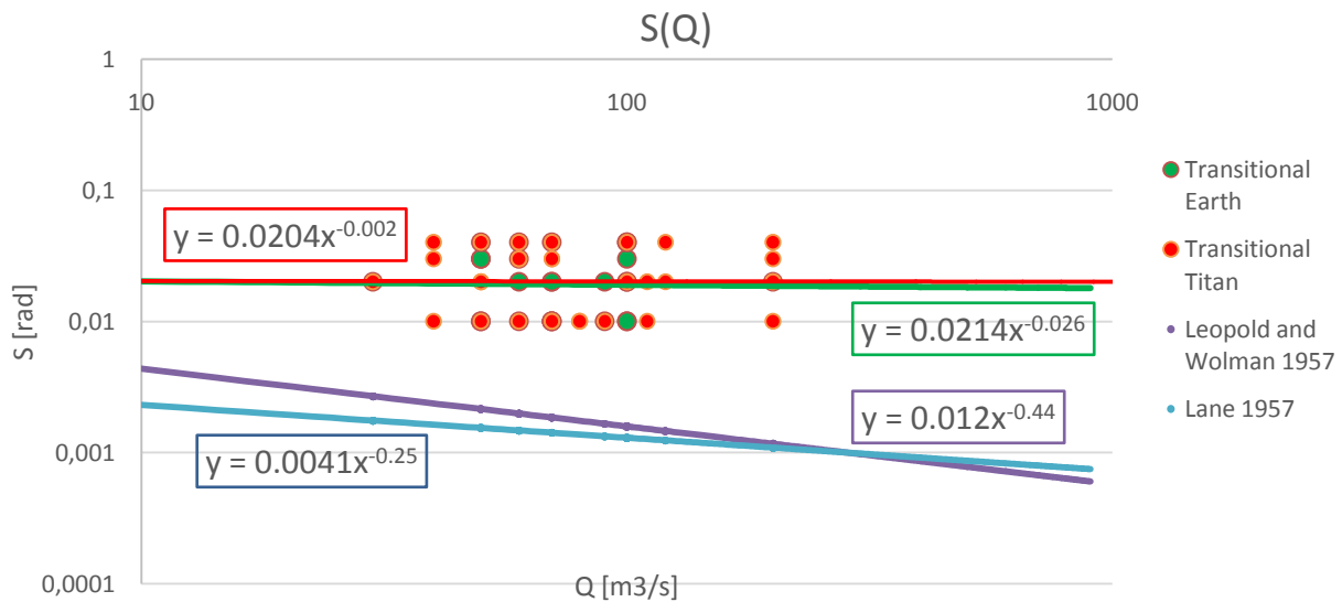
Fig. 2 Positions of simulated, transitional rivers and their trend lines (a power function) for Earth (green line) and Titan (red line) in space (S,Q) , for all considered S . There are shown also braiding and meandering predictors of Lane (1957) and Leopold and Wolman (1957) – lines purple and blue.
