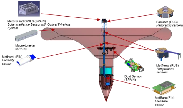
Figure 1: MetNet Lander strawman payload scheme.
