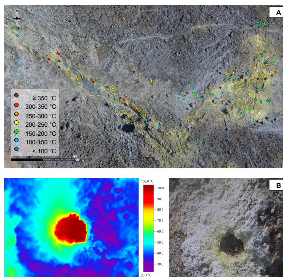
Figure 1: (A) High resolution drone based photogrammetry model and image mosaic with an overlay of the maximum measured temperatures at the mapped fissures; (B) example of an IR image (left) and associated RGB image (right) acquired during the 2017 field campaign.
