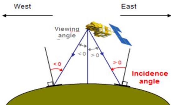
Figure 2. Representation of Viewing and Incidence angles (Courtesy of ASTRIUM DS France).
