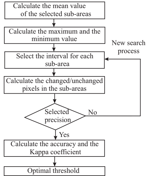
Figure 4: Flowchart of the proposed threshold determination algorithm.
