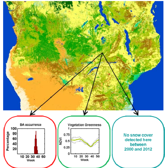
Figure 7. Climatological 7-day time series describing consistently and on a per-pixel basis the natural variability of the vegetation (NDVI), the snow cover and the burned areas
