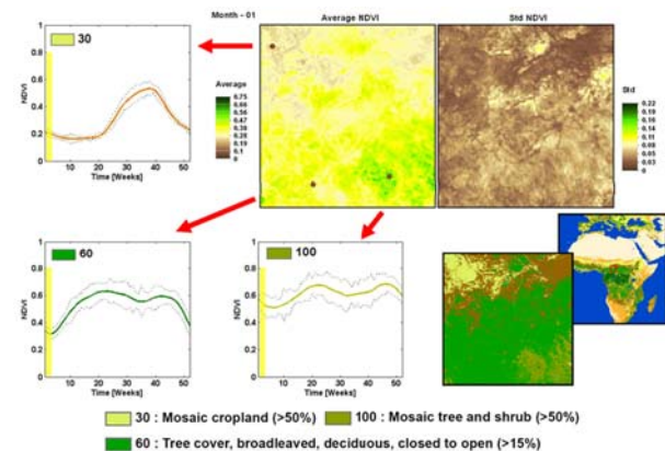
Figure 8. Detailed spatial example of NDVI climatological profiles - mean (plain line) and standard deviation (dotted line) - extracted in a region of Central Africa.
