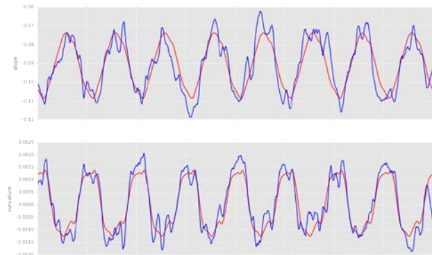
Figure 7: Yearly slope / curvature (red) versus daily slope / curvature (blue) estimates
