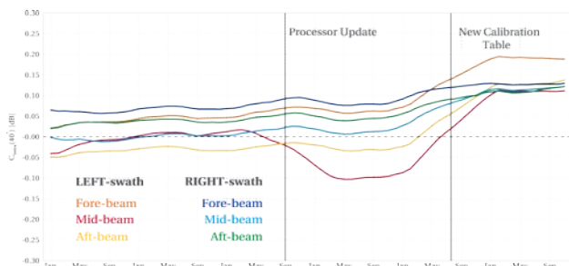
Figure 1: Radiometric stability of ASCAT from 2007 to 2013
