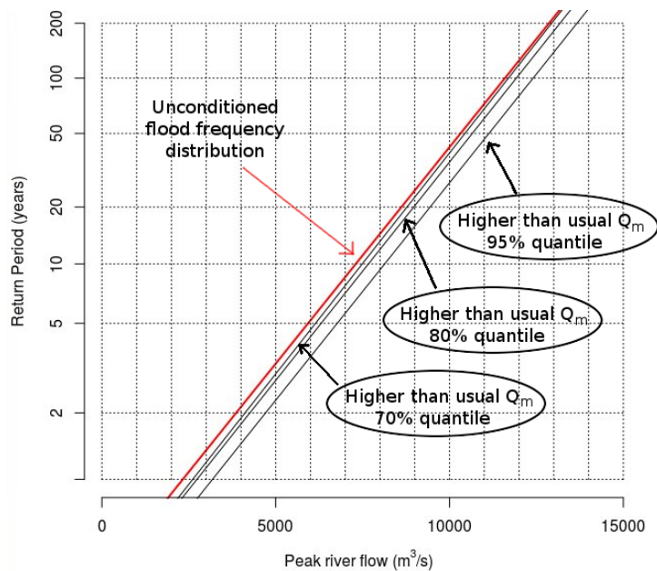
Figure 4. Peak flows in the flood season (Oct-Nov) vs return period modeled through the EVI distribution function.
