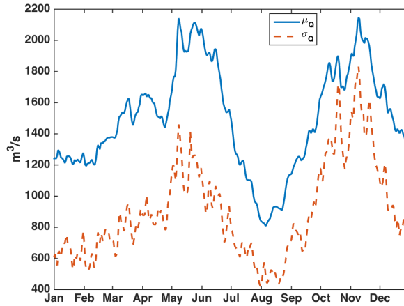
Figure 2. Daily mean value \mu_Q ( \text{m}^3\text{s}^{-1} ) and daily standard deviation \sigma_Q ( \text{m}^3\text{s}^{-1} ) of the daily flows in the observation period (1920-2009) at Pontelagoscuro
