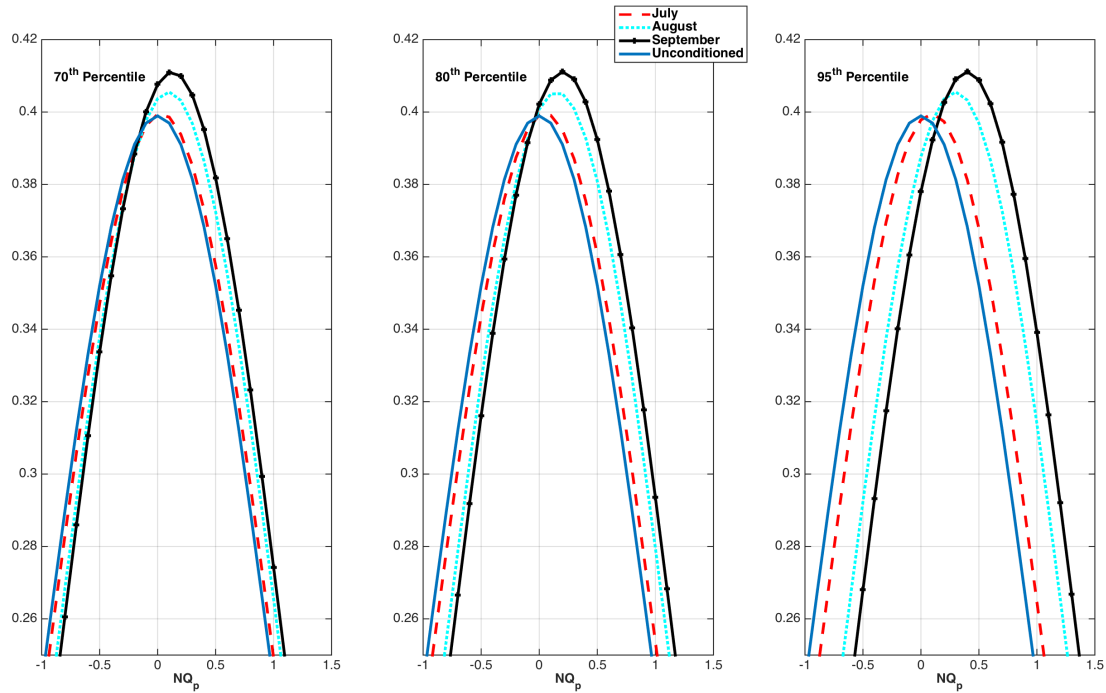
Figure 3. Probability distribution functions of the normalized dependent variable ( NQ_p ) conditioned to the occurrence of the 70 th , 80 th and 95 th percentiles of the normalized variables in the pre-flood season.
