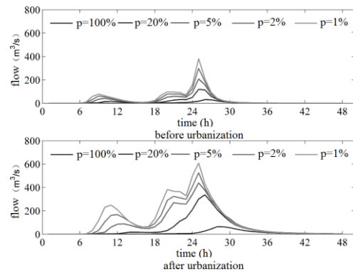
Fig. 7 Changes of floods in different urbanization scenarios
