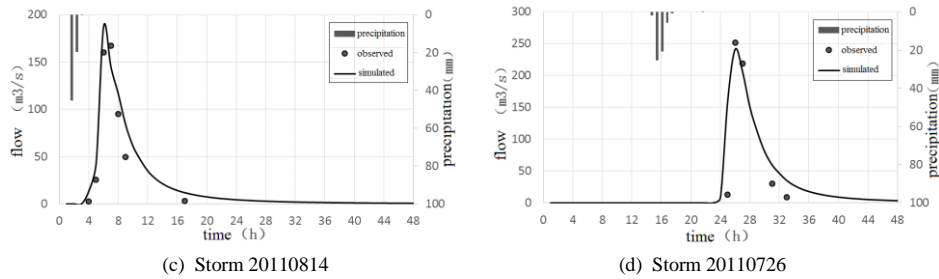
Fig. 5 Simulation of flood after urbanization
