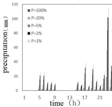
Fig. 6 24 hour-rainfall processes at different frequency
